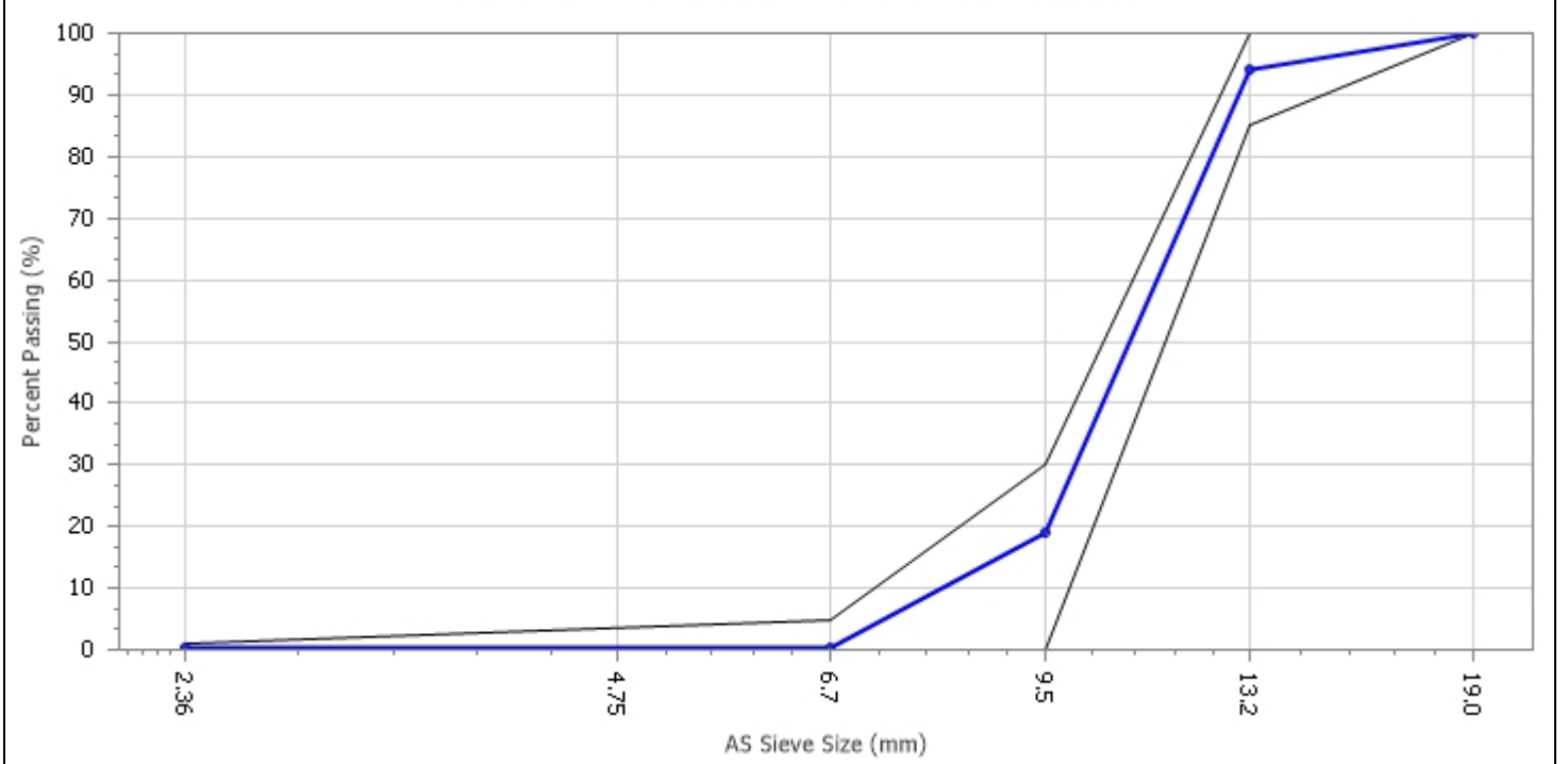
PARTICLE SIZE DISTRIBUTION GRAPH - 1692/S/22044
